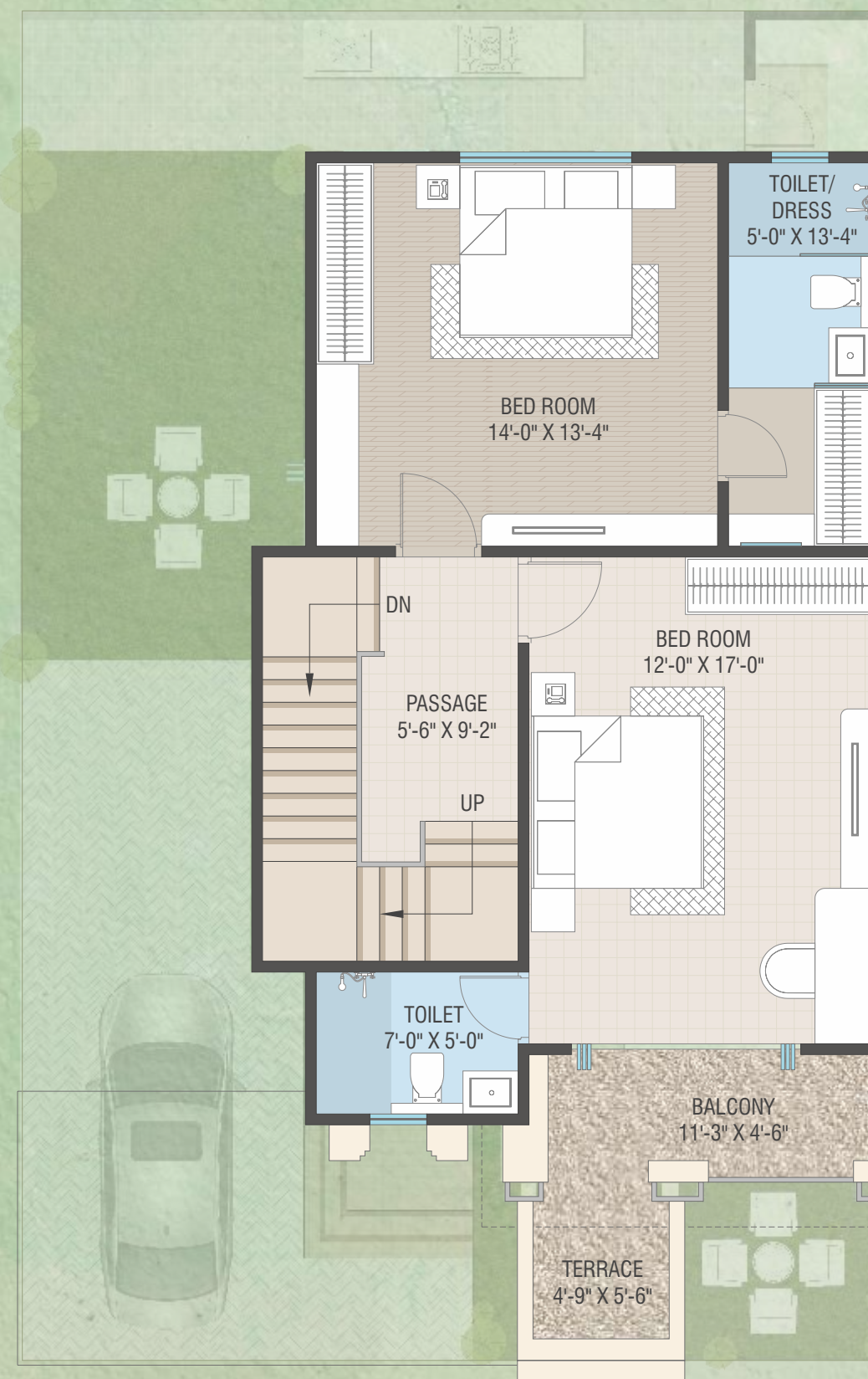
First floor
