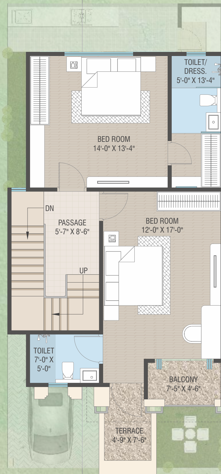
First floor
