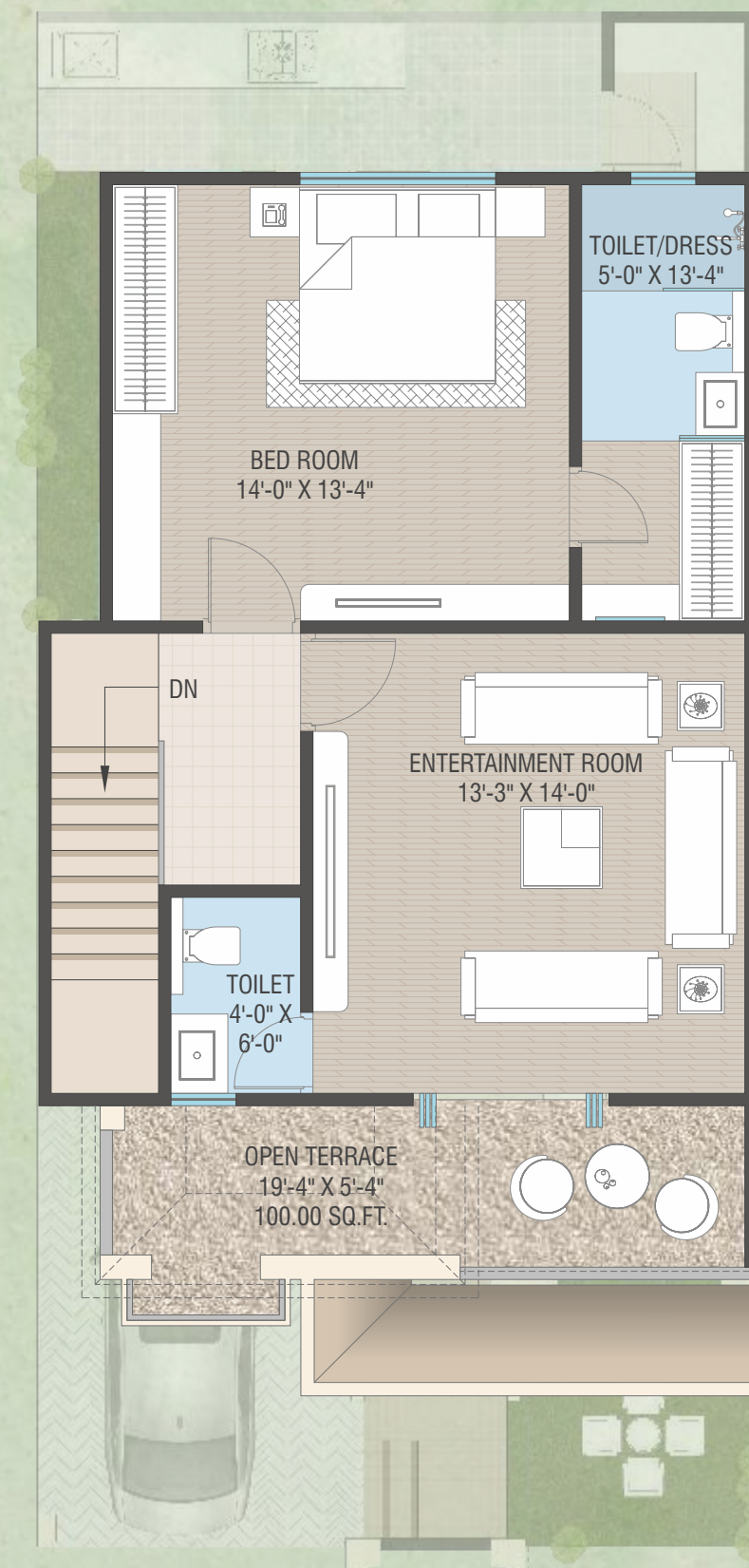
Second floor
